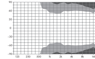
Y10P and Yi10P horizontal dispersion characteristics 2
