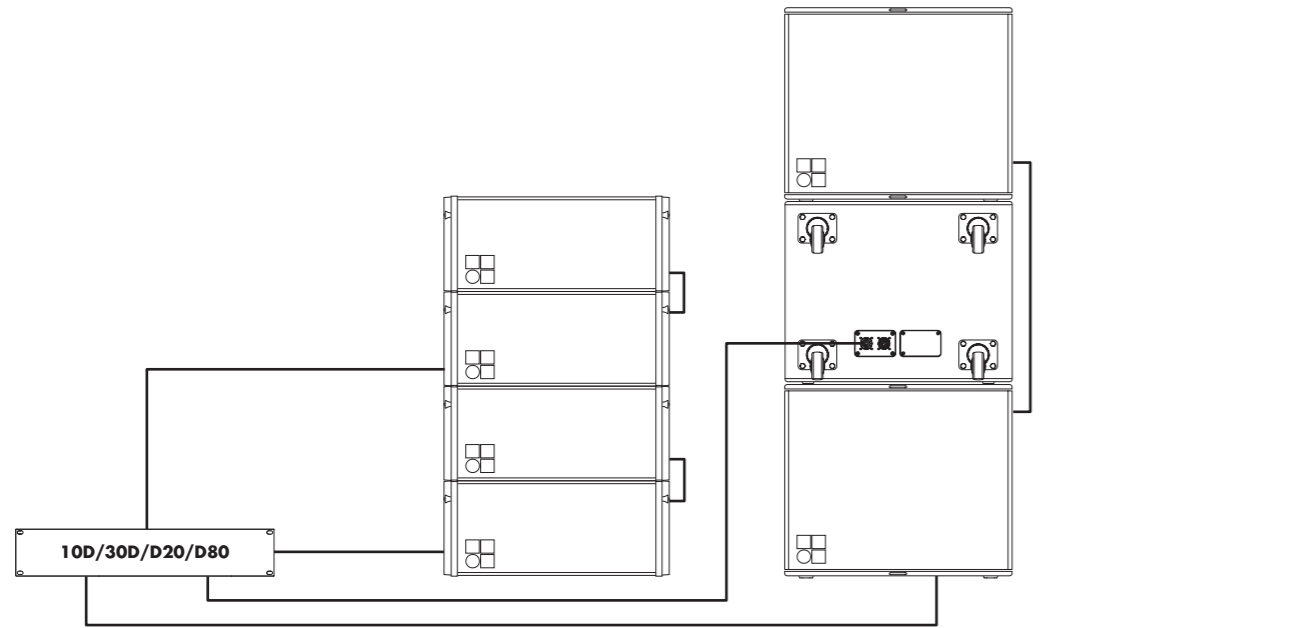
10D/30D/D20/D80 amplifier in Dual Channel mode for Y7P, Y10P, Yi7P, Yi10P, Y8, Y12, Yi8, Yi12 as well as B6-SUB, Bi6-SUB, Y-SUB and Yi-SUB (B6-SUB as CSA)
