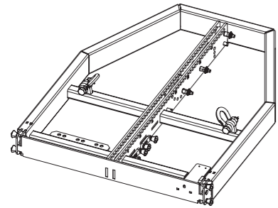
Z5390 Y Flying frame For a maximum of twenty four Y8/Y12/Yi8/Yi12 loudspeakers or ten Y/Yi subwoofers
