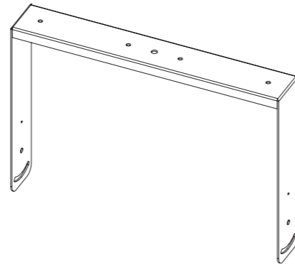
Z5389 Bi6-SUB Horizontal bracket
