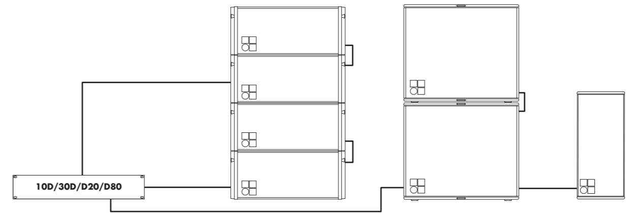
10D/30D/D20/D80 amplifier in a mixed configuration of Dual Channel and Mix TOP/SUB mode for Y7P, Y10P, Yi7P, Yi10P, Y8, Y12, Yi8 or Yi12 and B6-SUB, Bi6-SUB, Y-SUB or Yi-SUB
