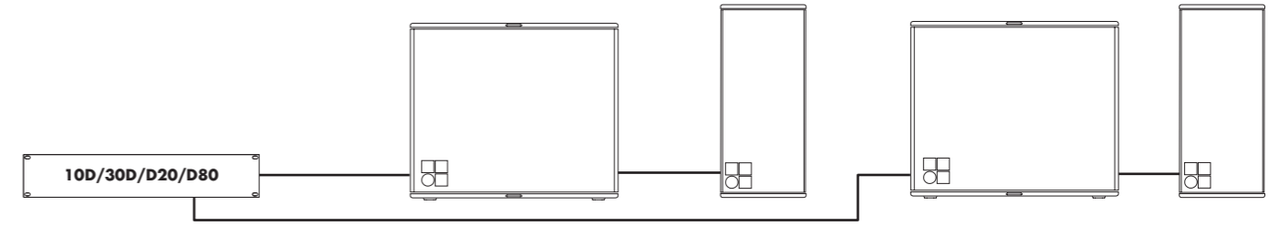
10D/30D/D20/D80 amplifier in Mix TOP/SUB mode for Y7P, Y10P, Yi7P, Yi10P, Y8, Y12, Yi8 or Yi12 and B6-SUB, Bi6-SUB, Y-SUB or Yi-SUB
