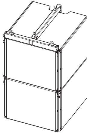
Yi-SUB column with Z5393.000 Y Mounting frame top
