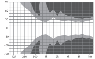
Y10P and Yi10P vertical dispersion characteristics 2
