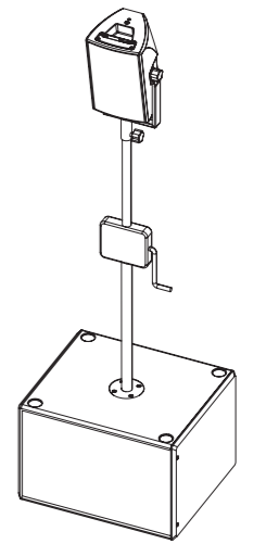
E6 with Z5377 E6 Swivel bracket Z5034 Stand adapter M10 Z5013 Stand winder M20
