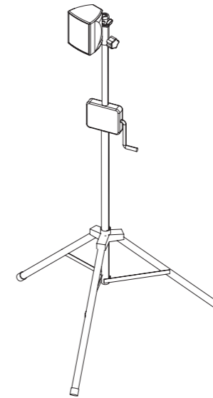
E4/E5 with Z5356 Ball joint adapter Z5034 Stand adapter M10 Z5009 Loudspeaker stand with winder
